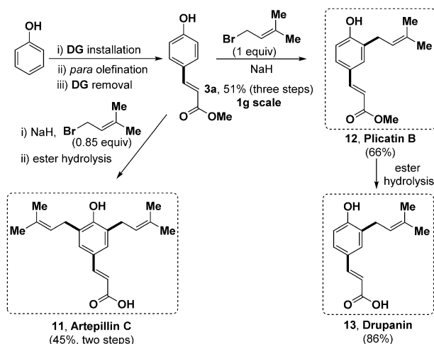
Scheme 4. Synthesis of artemillin C, plicatin B, and drupanin. [16]
