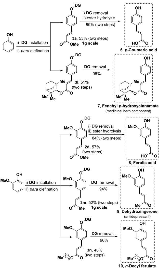
Scheme 3. Synthesis of phenol-based natural products. [16]
