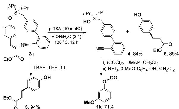
Scheme 2. Template removal and reinstallation. [16] DMAP = 4-dimethylaminopyridine, p-TSA = para -toluenesulfonic acid, TBAF = tetrabutylammonium fluoride.
