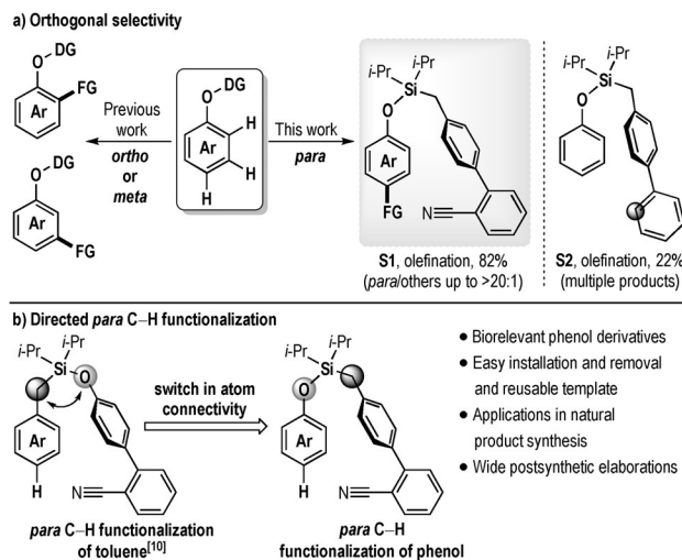
Scheme 1. Directed para C–H functionalization of phenols.
