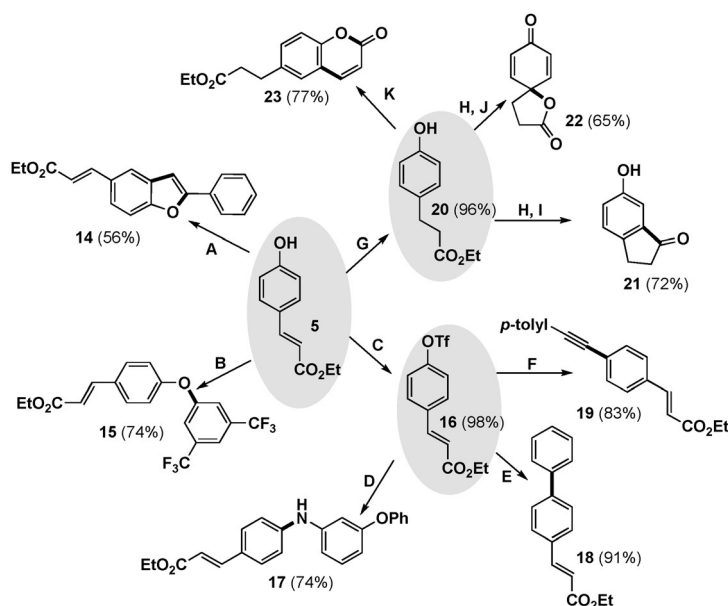
Scheme 5. Postsynthetic modifications. [16] A) Pd(OAc) 2 , 1,10-phenanthroline, styrene; B) CuI, picolinic acid, aryl iodide; C) Tf 2 O, K 3 PO 4 ; D) Pd 2 (dba) 3 , dppe, 3-phenoxylaniline; E) Pd(PPh 3 ) 4 /PhB(OH) 2 ; F) Pd(OAc) 2 , PPh 3 , para -tolylacetylene; G) Pd on C, H 2 ; H) LiOH; I) AlCl 3 , NaCl; J) PIFA; K) Pd catalyst, methyl acrylate. dba = dibenzylideneacetone, dppe = 1,1'-bis(diphenylphosphino)ferrocene, PIFA = (bis(trifluoroacetoxy)iodo)benzene, Tf = trifluoromethanesulfonyl.
